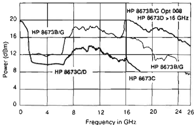
Figure 1. Maximum power typically available from HP 8673B/C/D/G and HP 8673B/G Option D08 at 25°C. HP 8673E and HP 8673H Option 212 and Option 618 typical maximum power is the same as HP 8673B/G over 2.0 to 18.0 GHz.
