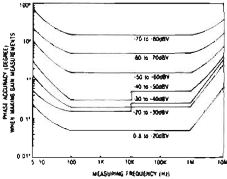
FIGURE 7: PHASE ACCURACY WHEN MEASURING GAIN MEASUREMENTS
