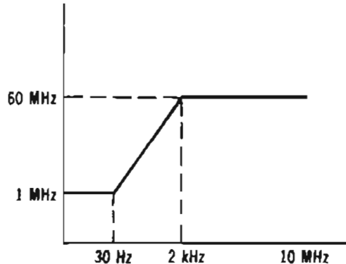
Figure 6 HP 5358D FM Tolerance
