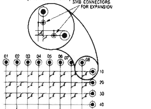
Switched-Shield Coaxial Multiplexer (one bank shown)
