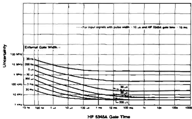
Graph 3. Uncertainty due to jitter (rms jitter) and gate error (\frac{.04}{EXT\ GATE\ WIDTH}) \pm 3\ kHz
