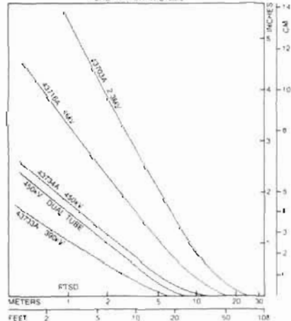
PENETRATION IN STEEL
