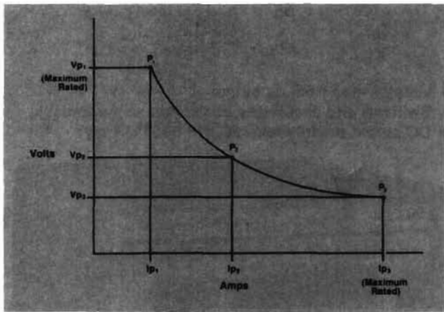
Generalized autoranging output characteristic curve Warranty period: Three years.
