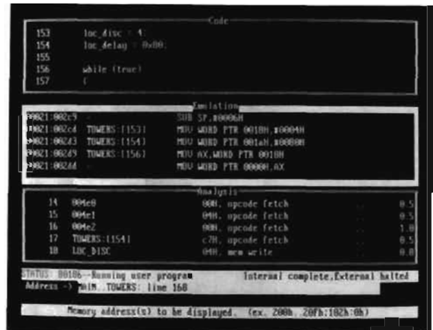
Source-line symbols help correlate memory and analysis displays with high-level code.
