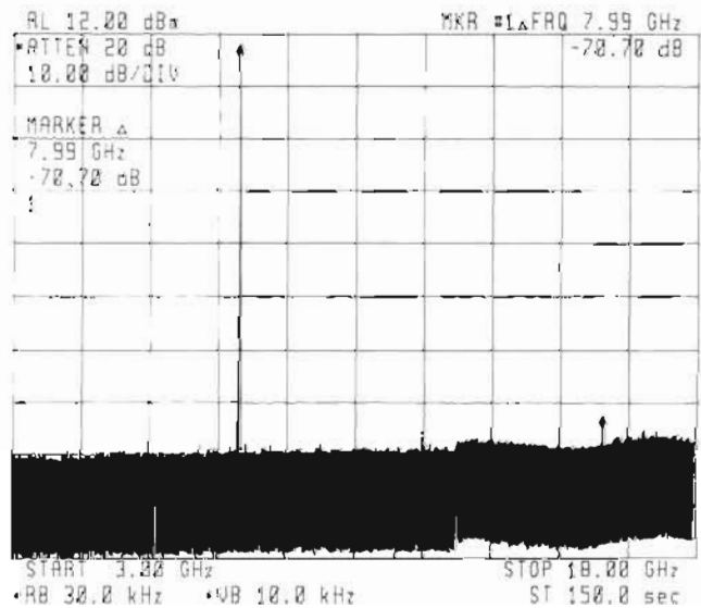
Harmonic Performance of the HP 83620A
