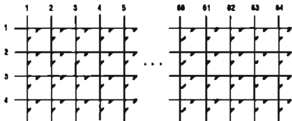
HP 34516N Two-Wire 256 Crosspoint Matrix
