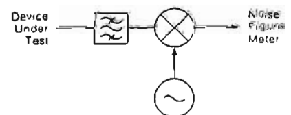
Single sideband noise measurement system.
