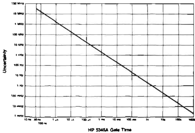
Graph 1. Uncertainty (2 x LSD) due to selected 5345A gate time.
