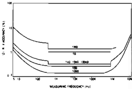
FIGURE 10: L, R ACCURACY
