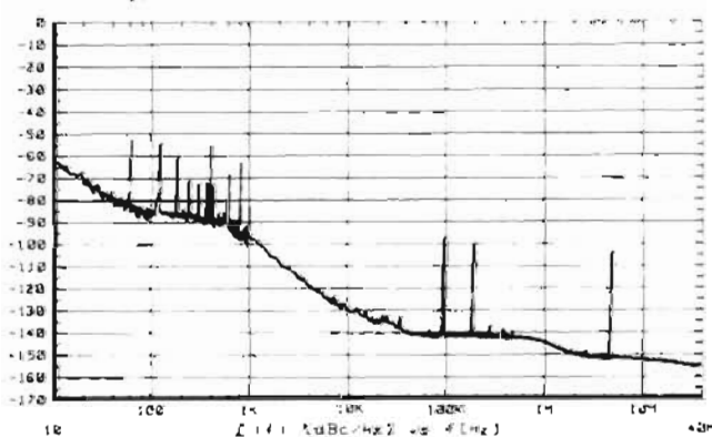
Typical HP 8657A SSB Phase-noise at 520 MHz
