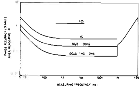
FIGURE 9: PHASE ACCURACY WHEN MEASURING L
