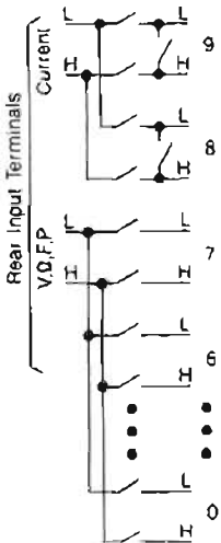
Armature Relay (44491A)
